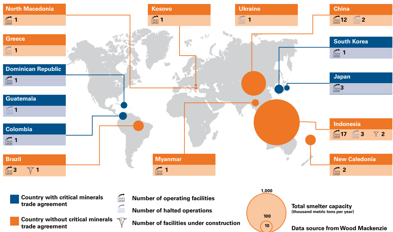
Figure 4: Total production capacity for ferronickel and nickel pig iron smelting, and number of existing smelting facilities by country
