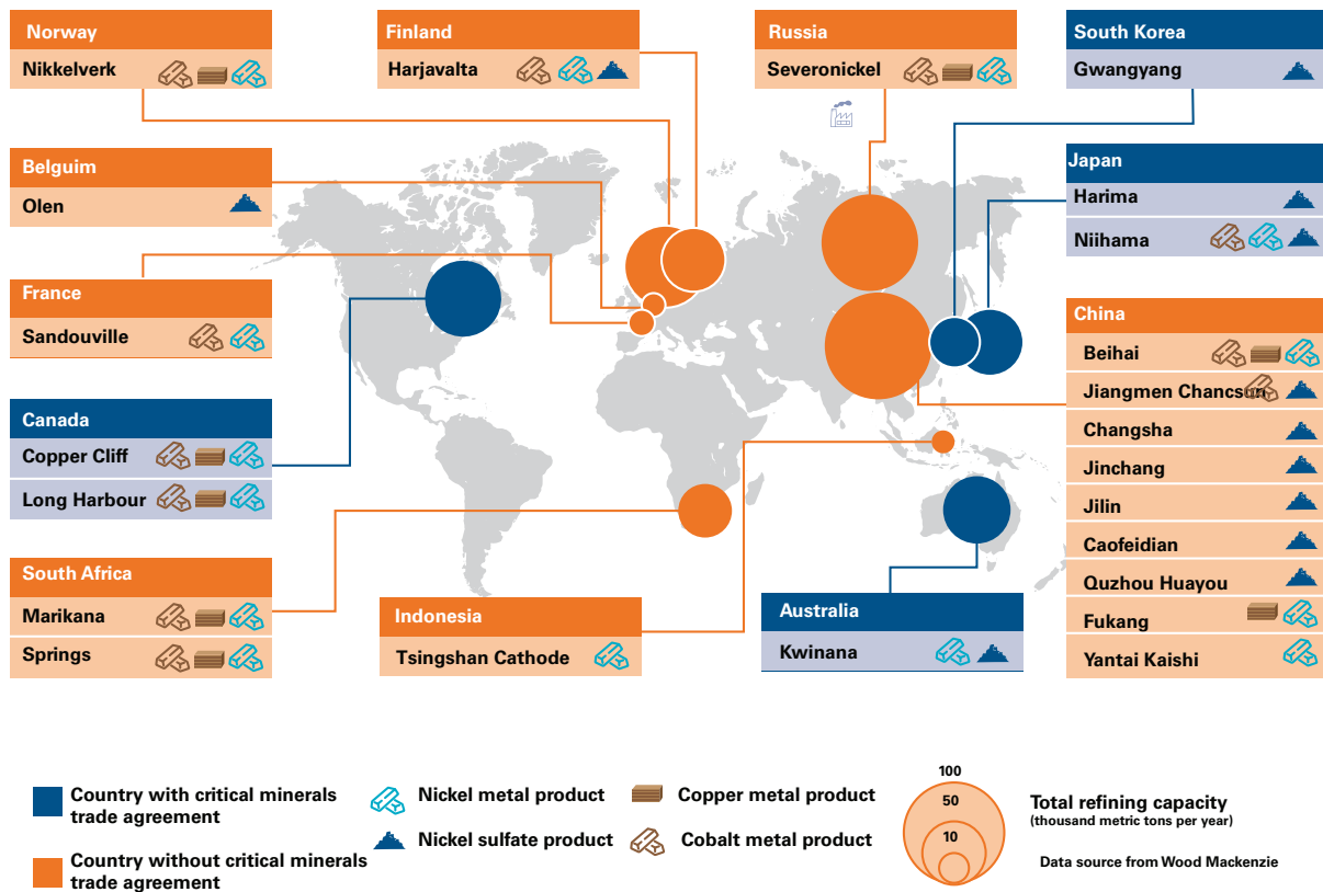
Figure 6: Total production capacity by country for products refined from matte, and product types by refining facility
