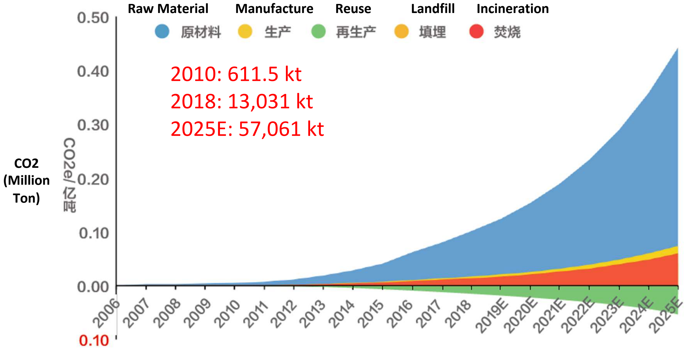
图 3-1 2006-2025 年快递包装全生命周期的碳排放 Figure 3-1 Carbon Emissions in Delivery Packaging's Life Cycle
